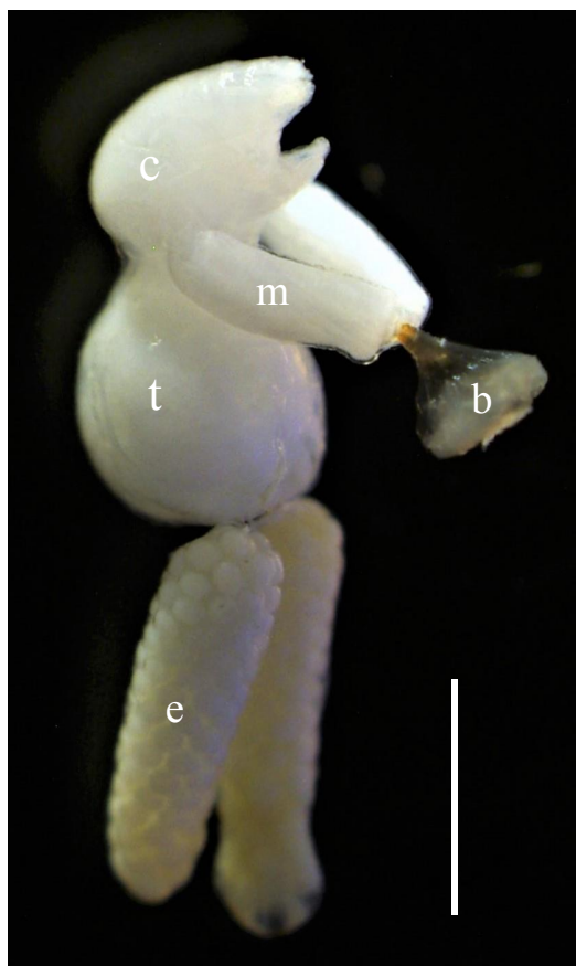
Fig. 1. Salmincola californiensis , adult female, from amago Oncorhynchus masou ishikawae in the Kami-Kurosawa Stream, a tributary of the Ôtaki River, Nagano Prefecture, central Japan. Alcohol-preserved specimen, ventrolateral view. b, bulla; c, cephalothorax; e, egg sac; m, maxilla; t, trunk. Scale bar: 2 mm.
