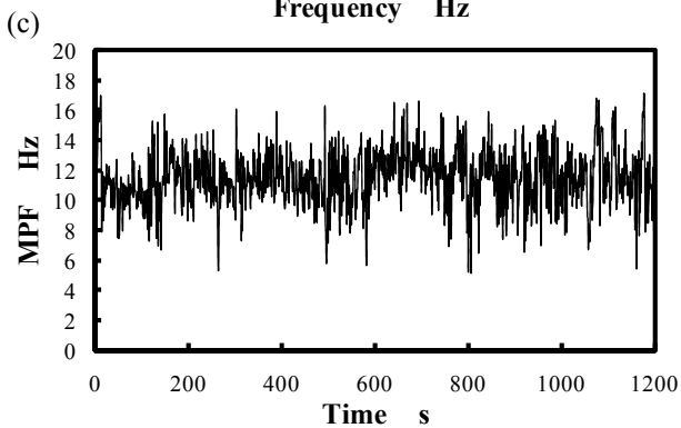
Fig.2 (a) Time series of EEG wave form, (b) An example of EEG power spectrum, (c) Time series of MPF.
