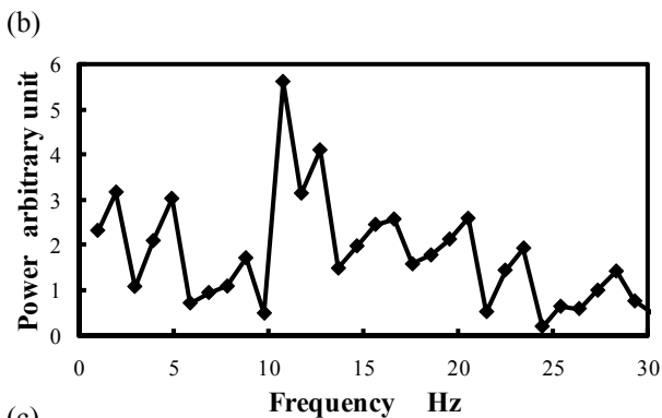
Fig.3 Comparison of MPF before and after the warning sounds.
