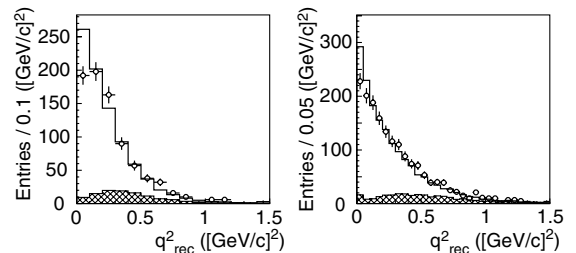
FIG. 1. The q_{\text{rec}}^2 distributions for 2-track non-QE samples of SciFi (left) and SciBar (right). Open circles, solid lines, and hatched areas show data, MC predictions, and the CC-QE component estimated from MC simulation, respectively.
