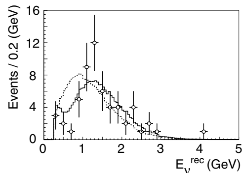
FIG. 3. The reconstructed E_\nu^{\text{rec}} distribution for the SK 1-ring \mu -like sample. Points with error bars are data. The solid line is the best fit spectrum. The dashed line is the expected spectrum without oscillation. These histograms are normalized by the number of events observed (57).
