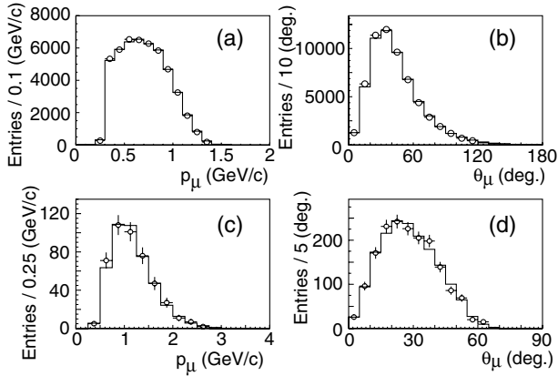
FIG. 2. A selection of muon momentum ( p_\mu ) and direction ( \theta_\mu ) distributions: (a) the p_\mu distribution of the 1KT fully contained 1-ring \mu -like sample, (b) 1KT \theta_\mu for the same sample, (c) SciFi p_\mu for the 2-track QE sample, and (d) SciBar \theta_\mu for the 2-track non-QE sample. Open circles represent data, while histograms are MC predictions using the best fit E_\nu spectrum and suppression of the resonant pion production.
