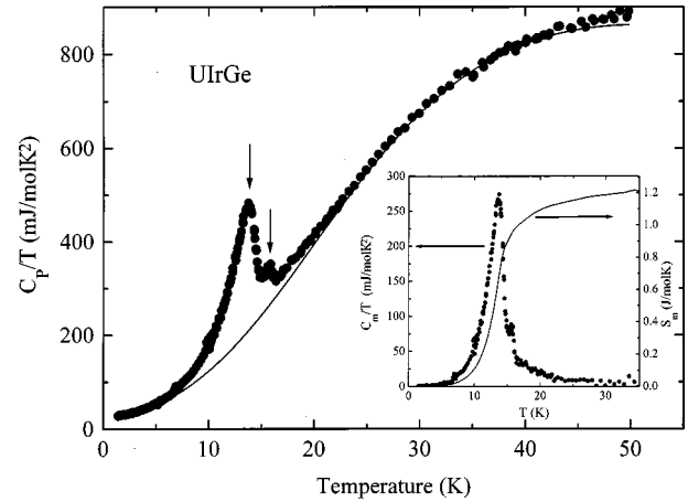
FIG. 3. The temperature dependence of the specific heat of UIrGe in zero field divided by temperature C_p/T . The solid line represents the sum of the electronic contribution (given by the low-temperature specific-heat coefficient \gamma = 25.69 mJ/mol K 2 ) and the phonon part approximated by a Debye function with \theta_D = 182 K. In the inset, the temperature dependence of the magnetic part of the specific heat divided by temperature together with the magnetic entropy is shown.
