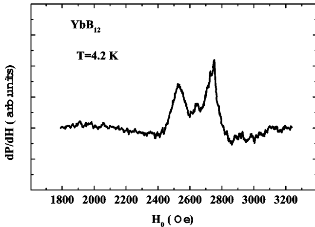
FIG. 1. ESR spectrum at T=4.2 K and \phi=0^\circ demonstrating two large lines and a weak in-between line.
