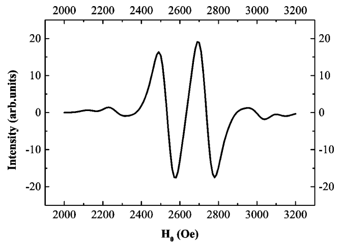
FIG. 6. Computer simulation of the ESR signal for \phi=0^\circ with hyperfine structure included both for 171 Yb and 173 Yb isotopes. The linewidth was set to 60 Oe.
