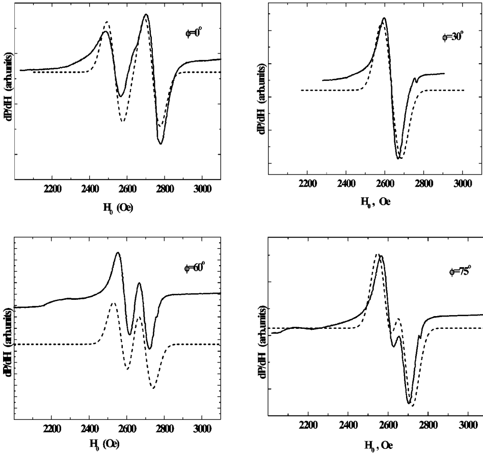
FIG. 3. ESR spectra for four values of the angle \phi between the magnetic field and [001] direction in the (110) plane. Solid lines are experimental spectra; dashed lines are calculated ones.
