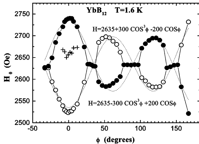
FIG. 4. Angular dependence of the ESR lines position for rotation of the magnetic field in the (110) plane. Additional points at 2650–2675 Oe are due to unpaired \text{Yb}^{3+} ions.
