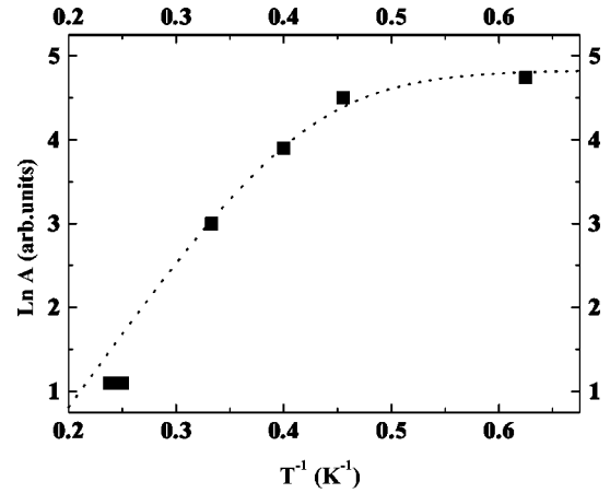
FIG. 5. Temperature dependence of the maximum-to-minimum amplitude of the ESR line for \phi = 90^\circ . Dotted curve is drawn according to the relation D/[1 + R \exp(-\Delta/T)] with D = 125 , R = 2000 , and \Delta = 18 K.
