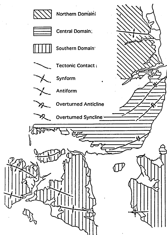
Fig. 2 Structural domains (northern, central, and southern domains) in the Yanai district. Axial traces of major folds are also illustrated.
