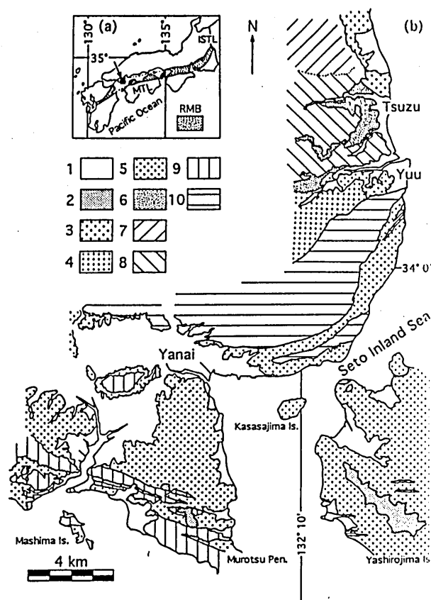
Fig. 1 (a) Outline map showing the location of the Ryoke metamorphic belt of southwest Japan. RMB: Ryoke metamorphic belt. MTL: Median Tectonic Line. ISTL: Itoigawa-Shizuoka Tectonic Line. (b) Geological and metamorphic zonation map of the Yanai district, southwest Japan. 1: alluvium. 2: Tertiary volcanics. 3: Iwakuni granite. 4: Kibe granite. 5: Gamano granodiorite. 6: Tengatake-Nagano migmatite. 7 - 10 : Ryoke metamorphic rocks (7 biotite zone, 8 cordierite zone, 9 sillimanite zone, 10 garnet zone).
