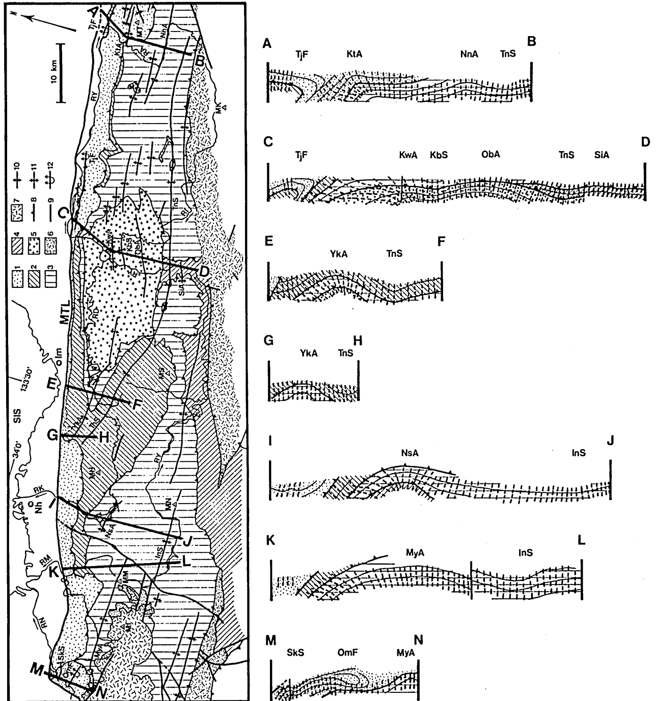
Fig. 4. Schematic diagram showing the orientation pattern of Sh in the large-scale Dh phase folds along seven cross sections.
