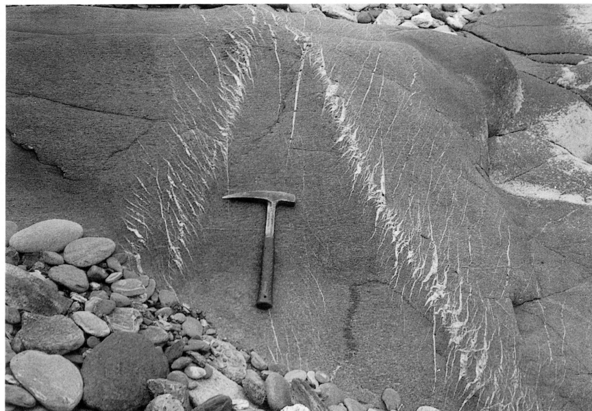
Fig. 10. En echelon quartz veins developed as conjugate sets in the Sambagawa schist (psammitic schist) of Shimomyo along the River Yoshino.
