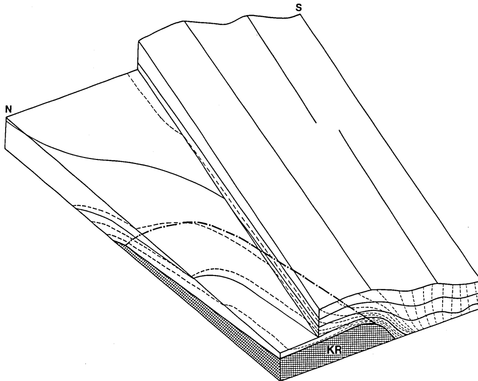
Fig. 9. Schematic diagram showing the orientation pattern of Sh in the large-scale Dh phase folds and of the rigid body tectonically emplaced beneath the Sambagawa schists. dashed lines: Sh, KR: tectonically emplaced rigid body.
