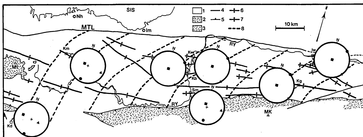
Fig. 12. Diagram showing the localities of the data of Fig. 11 and the orientation directions of the stress axes assumed from Fig. 11.
