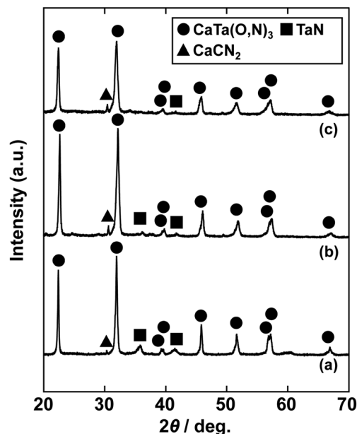
Fig. 2 XRD patterns of products prepared from \text{CaCO}_3 , \text{Ta}_2\text{O}_5 gel, and urea after heat treatment at 950\text{ }^\circ\text{C} for 2 h. Molar ratios of Ca/Ta/urea in precursors were (a) 1:1:5, (b) 1.5:1:5 and (c) 2:1:5.
