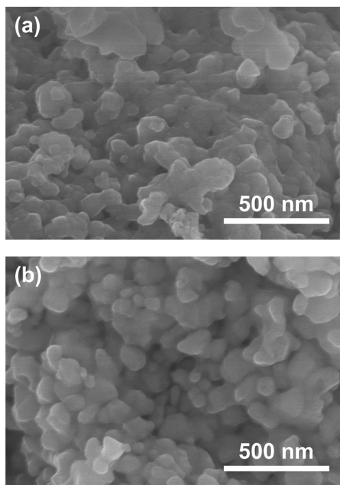
Fig. 5 SEM images of \text{CaTa}(\text{O},\text{N})_3 prepared from Ca source (a) \text{CaCO}_3 , (b) \text{Ca}(\text{OH})_2 , \text{Ta}_2\text{O}_5 gel and urea after heat treatment at 950^\circ\text{C} for 2 h. Molar ratios of Ca/Ta/urea in precursors were (a) 2 : 1 : 5 and (b) 1.5 : 1 : 3.
