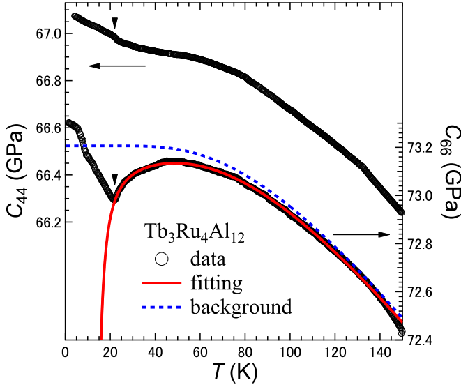
FIG. 3. T dependencies of the transverse elastic moduli C_{44} and C_{66} in \text{Tb}_3\text{Ru}_4\text{Al}_{12} . The vertical arrow indicates the phase transition at T_N . The red solid and blue broken curves represent the fitting result and the background stiffness, respectively.
