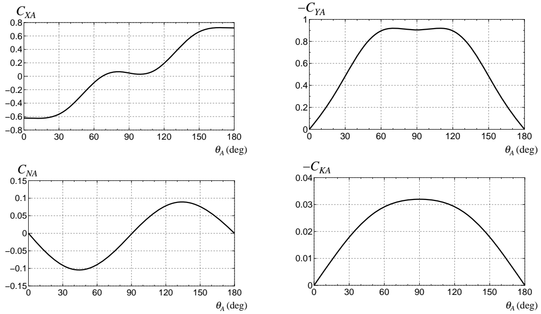
Fig. 5: Aerodynamic force coefficients
