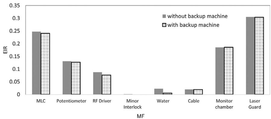
FIG. 8. EIR_{MF} for machine failures caused by MLC, potentiometer, RF driver, minor interlock, water temperature and quantity, cable, monitor chamber, and LaserGuard with and without backup machine.
