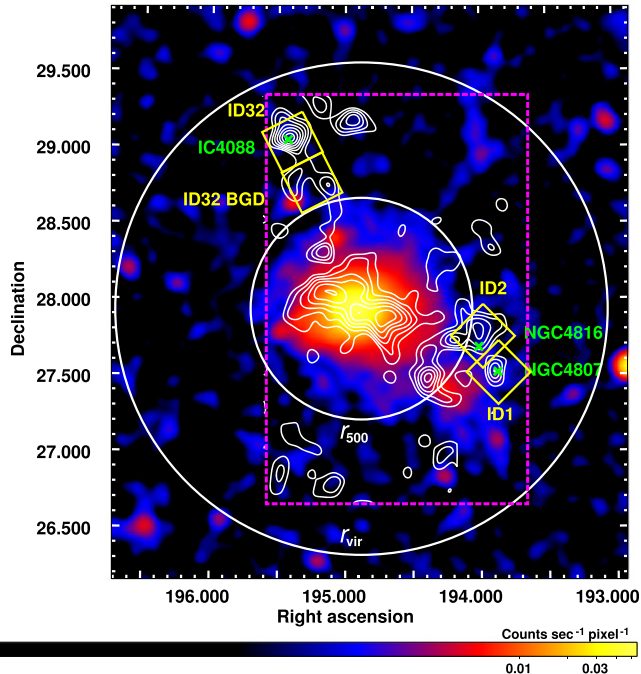
Figure 1. Weak-lensing mass contour map in linear scale from Subaru overlaid on the X-ray image taken by the ROSAT All Sky Survey in the 0.1–2.4 keV band. Here, the exposure time was corrected and instrumental backgrounds were subtracted. The X-ray image was smoothed by a Gaussian of \sigma \approx 2' . The color bar is in units of counts s^{-1} pixel ^{-1} . The FOVs of the Suzaku pointings are plotted with boxes (yellow). The solid (white) circles indicate r_{500} ( \sim 44' ) and r_{vir} \sim r_{98}(\sim 97') , respectively, which were derived with weak-lensing observations by Okabe et al. (2010). The dashed (magenta) box shows the field of the Subaru weak-lensing survey (Okabe et al. 2014a) and the mass distribution derived from this survey was overlaid in contours. The crosses (green) show the positions of representative galaxies, NGC 4807, the NGC 4816 group, and IC 4088, for the subhalos “ID 1,” “ID 2,” and “ID 32,” respectively.
