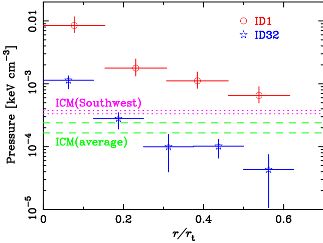
Figure 6. Thermal pressure profile of “ID 1” centered on the mass center (open circles) and that of “ID 32” centered on the X-ray peak (open stars). The dotted (magenta) and dashed (green) lines indicate the ICM pressure range of the southwest direction and azimuthal average excluding the southwest direction derived by Simionescu et al. (2013).
