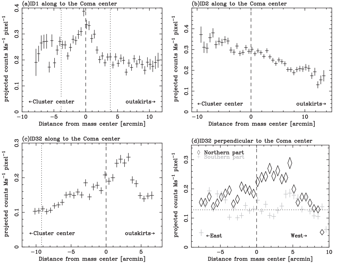
Figure 3. Projected surface brightness profiles of (a) “ID 1” subhalo, (b) “ID 2” subhalo, and (c) “ID 32” subhalo along the direction to the outskirts from the Coma cluster center extracted from the combined XIS FOV images in the 0.5–2.0 keV energy band. The side of the negative numbers corresponds to the direction to the center of the Coma cluster. Here, the NXB was subtracted and the effect of the exposure time and vignetting were corrected. The minus X -axis corresponds to the direction of the Coma cluster center. The dashed vertical lines indicate the center of each subhalo and the dotted vertical lines show the truncation radius of the subhalo “ID 1” and “ID 32.” (d) The projection direction is perpendicular to (c). The sides of the negative and positive numbers correspond to the directions east and west.
