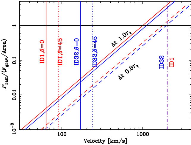
Figure 8. Ratio of the ram pressure to gravitational force per area against the velocity of each subhalo. The solid and dashed lines are the ratio calculated at 1.0 r_t and 0.6 r_t , respectively. The red and blue lines correspond to “ID 1” and “ID 32,” respectively. The vertical solid and dotted lines correspond to velocities of each subhalo assuming the 0^\circ and 45^\circ inclination angle, respectively. The infall velocities are plotted with the red and blue dot-dashed lines for “ID 1” and “ID 32,” respectively. The horizontal solid line corresponds to unity.
