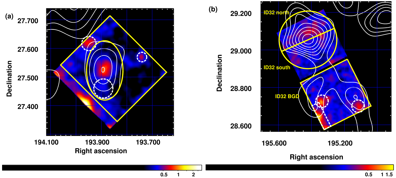
Figure 4. Same images as Figure 2. The elliptical region (yellow) in the left panel and semicircular regions (yellow) in the right panel are used in spectral extraction for the “ID 1” subhalo, and “south” and “north” regions of the “ID 32” subhalo, respectively. The solid box (yellow) in the left panel excluding the elliptical region and that in the right panel are used in the background analysis (“ID 1 BGD” and “ID 32 BGD,” respectively). The regions within the dashed box and circles (white) are excluded from these spectral analyses.
