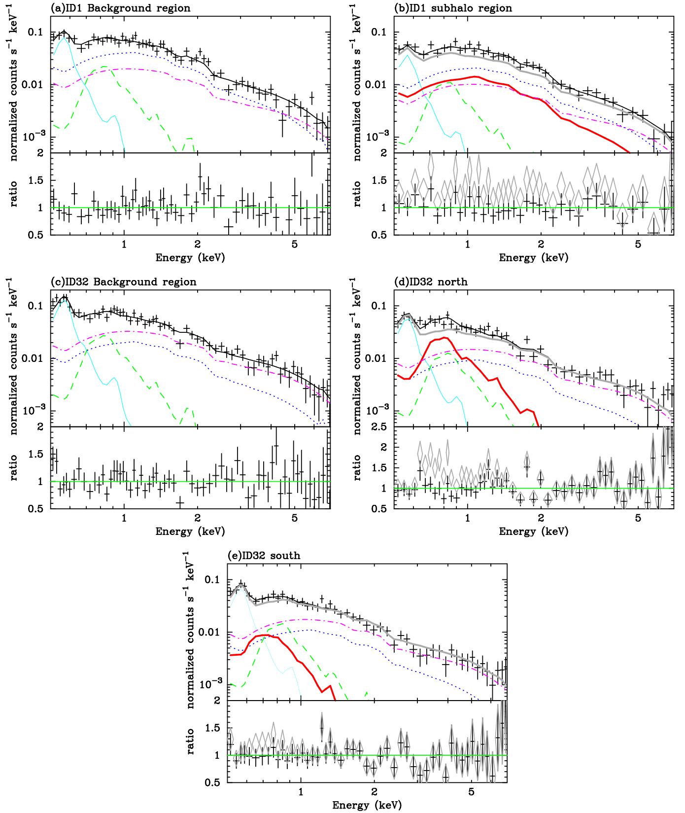
Figure 5. Spectra of (a) “ID 1 BGD,” (b) the subhalo region spectra of “ID 1,” (c) “ID 32 BGD,” and (d) and (e) “north” and “south” regions of the subhalo “ID 32,” respectively. The spectra were rebinned here for display purposes only. Upper panels show the NXB subtracted XIS 1 spectra (black crosses). The subhalo component is plotted by the (red) bold line. The ICM, CXB, LHB, and MWH components are indicated by (blue) dotted, (magenta) dash-dotted, (cyan) thin, and (green) dashed lines, respectively, and the gray solid line indicates the sum of these background components. The lower panels show the data-to-model ratios. The gray diamonds in the lower panels in (b), (d), and (e) show those without the subhalo component, in which the ratio indicates that the subhalo component cannot be negligible.
