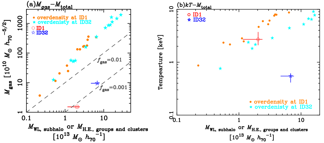
Figure 7. (a) The subhalo gas mass against weak-lensing mass or hydrostatic mass. The open (red) circles and (blue) stars indicate “ID 1” and “ID 32,” respectively. The error bars of the weak-lensing masses of the subhalos include the systematic errors. The filled (orange) circles and (cyan) stars are the gas mass vs. hydrostatic mass at the radius within which the mean density of the groups and clusters are the same overdensity as “ID 1” and “ID 32,” respectively. The gas mass and hydrostatic mass of the groups and clusters were calculated from Chandra ’s results (Vikhlinin et al. 2006). (b) The same as the left panel but for temperature vs. weak-lensing mass or hydrostatic mass.
