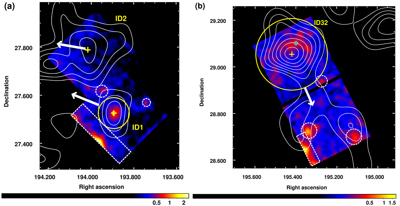
Figure 2. Weak-lensing mass contour map in linear scale overlaid on the NXB subtracted XIS images in 0.5–2.0 keV. (a) around “ID 1” and “ID 2,” and (b) around “ID 32” in the 0.5–2.0 keV energy band. Here, the difference in the exposure times and the vignetting effect at 1 keV were corrected. The images were smoothed by a Gaussian of \sigma = 24 pixels \approx 25'' . The numbers below the color bars have units of counts Ms -1 pixel -1 . The contours (white) show the mass map derived from weak-lensing by Okabe et al. (2014a). The direction of the Coma cluster center from the center of each subhalo is shown by the arrow. The crosses are the center of each subhalo as summarized in Table 1. For “ID 1” and “ID 32,” the solid (yellow) circles show the truncation radii. The diamond (cyan) mark in the “ID 32” subhalo corresponds to the X-ray peak of the excess emission. When creating the surface brightness profiles, the regions in the dashed (white) circles and boxes were excluded.
