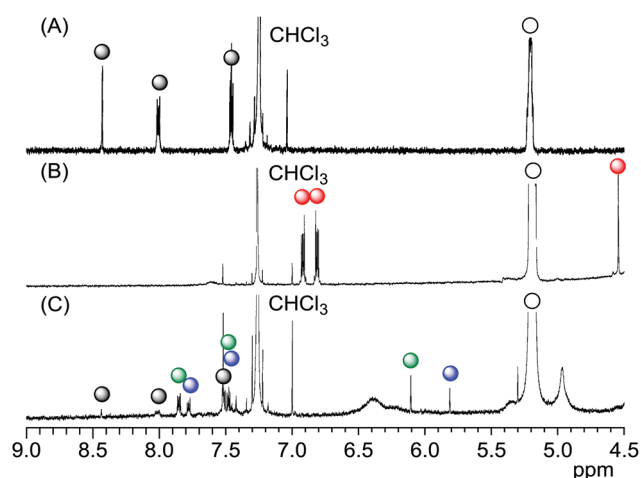
Fig. 3 Partial 1 H NMR spectra of (A) LMI1 (●: 1, ○: DMPC), (B) LMI1 after irradiation at 365 nm for 3 h ( 1.5 \text{ W m}^{-2} , ●: 1, ○: DMPC) and (C) LMI2 (●: 1, ○: DMPC) ([1] = 0.042 mM, [C_{60}] = 0.042 mM, [1]/[DMPC] = 1.4 mol%). All spectra were obtained using CDCl 3 solutions of freeze-dried samples.
