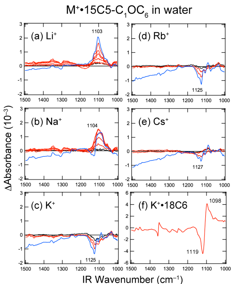
Figure 2. (a–e) The IR difference spectra of the \text{M}^+\cdot 15\text{C}5\text{-C}_1\text{OC}_6 ( \text{M} = \text{Li}, \text{Na}, \text{K}, \text{Rb}, \text{and Cs} ) complexes on the gold surface using aqueous MCl solutions. The concentration of the MCl salts in water ranges from 10^{-6} to 1 M for \text{Li}^+ and \text{Na}^+ and from 10^{-3} to 1 M for \text{K}^+ , \text{Rb}^+ , and \text{Cs}^+ . The blue
