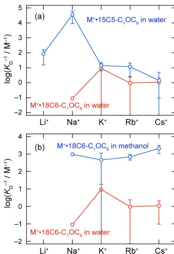
Figure 5. The reciprocal of the apparent K_D values determined by fitting the intensity around 1100 cm^{-1} in the IR difference spectra of (a) M^+ \cdot 15C5-C_1OC_6 in water and (b) M^+ \cdot 18C6-C_1OC_6 in methanol (blue circles). For comparison, the data of M^+ \cdot 18C6-C_1OC_6 in water are shown in both panels (red circles) (Ref. 10 ).
