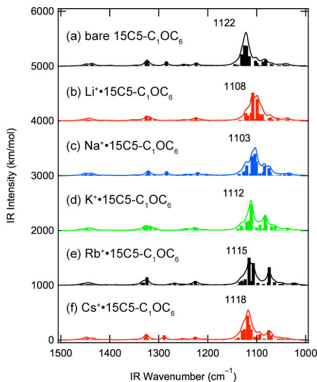
Figure 7. The IR spectra of the M^+ \cdot 15C_5-C_1OC_6-CH_3 ( M = Li, Na, K, Rb, and Cs ) complexes and bare 15C_5-C_1OC_6-CH_3 calculated at the M05-2X/6-31+G(d) level with the PCM of water. A scaling factor of 0.9389 is employed for the calculated vibrational frequencies. The solid curves are the IR spectra produced by providing a Lorentzian component with a FWHM of 10 \text{ cm}^{-1} to each band.
