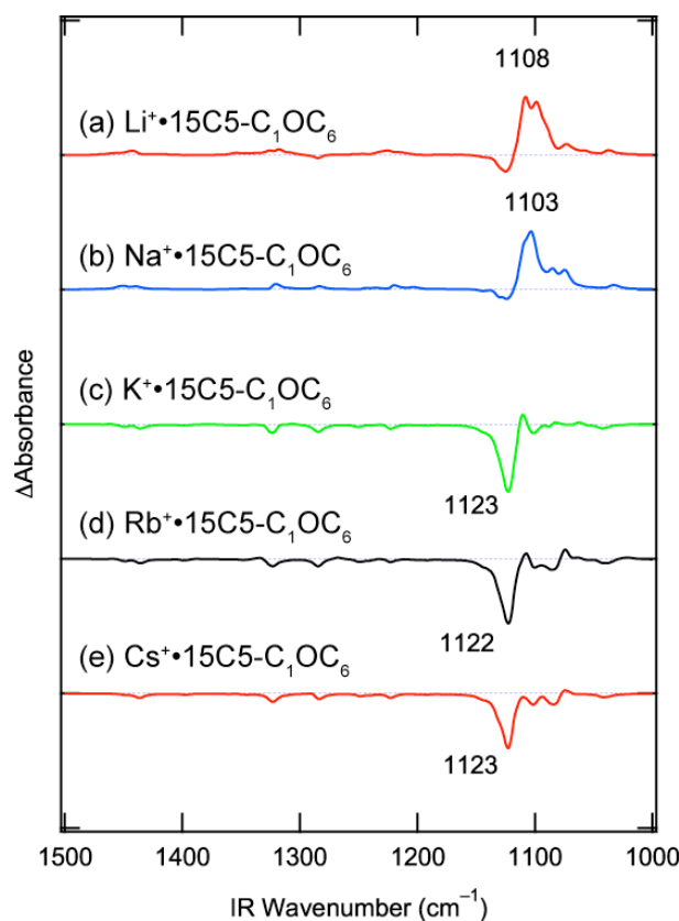
Figure 8. The IR difference spectra made by subtracting the simulated IR spectrum of bare 15C5-C_1OC_6-CH_3 in Fig. 7a from those of the M^+\cdot 15C5-C_1OC_6-CH_3 complexes in Figs. 7b–f. In the simulation of the Li^+ and Na^+ complexes, the calculated IR intensity of the M^+\cdot 15C5-C_1OC_6-CH_3 complexes is multiplied by 2 before the subtraction, while for the K^+ , Rb^+ , and Cs^+ spectra, the IR intensity of bare 15C5-C_1OC_6-CH_3 is multiplied by 2 (see text).
