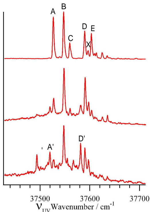
図1 L -Phenylalanine と水和クラスターの LIF スペクトル (a) no water (b) with water (at 0 ) (c) with water (at room temperature)
