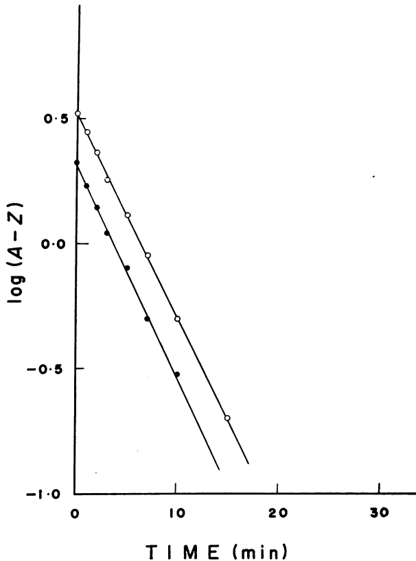
Text-fig. 15. Log (A-z) - t diagram for nitrogen-water.
