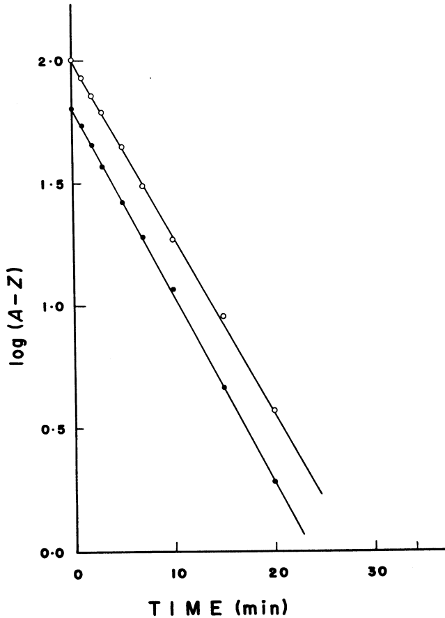
Text-fig. 7. Log (A-z) - t diagram for carbon dioxide-water
