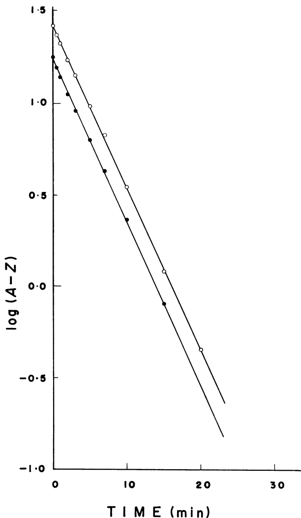
Text-fig. 12. \log(A-z) - t diagram for nitrogen-methyl oleate.
