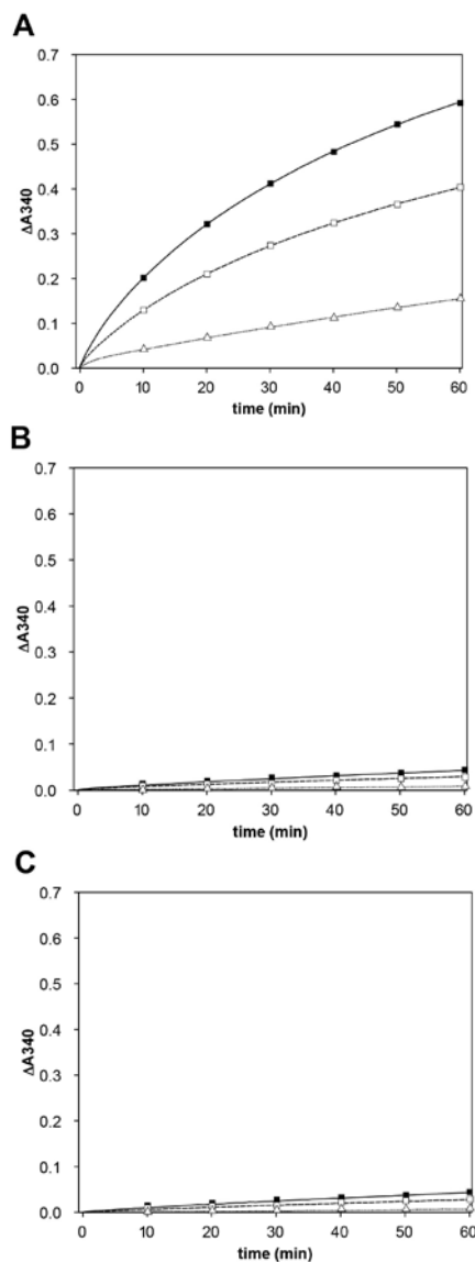
Fig. 2. NADPH-coupled assays for the (A) reduction of \text{V}^{\text{V}} , (B) reduction of \text{Mo}^{\text{VI}} , and (C) reduction of \text{W}^{\text{VI}} . Solid line with solid rectangles correspond to the reaction with 4 \mu\text{M} Vanabin2. Dashed line with open rectangles corresponds to the reaction with 2 \mu\text{M} Vanabin2. Dotted line with open triangles shows data acquired without Vanabin2. The horizontal axis indicates the time after initiation of the reaction. The vertical axis indicates the decrease in absorbance at 340 nm due to NADPH oxidation.
