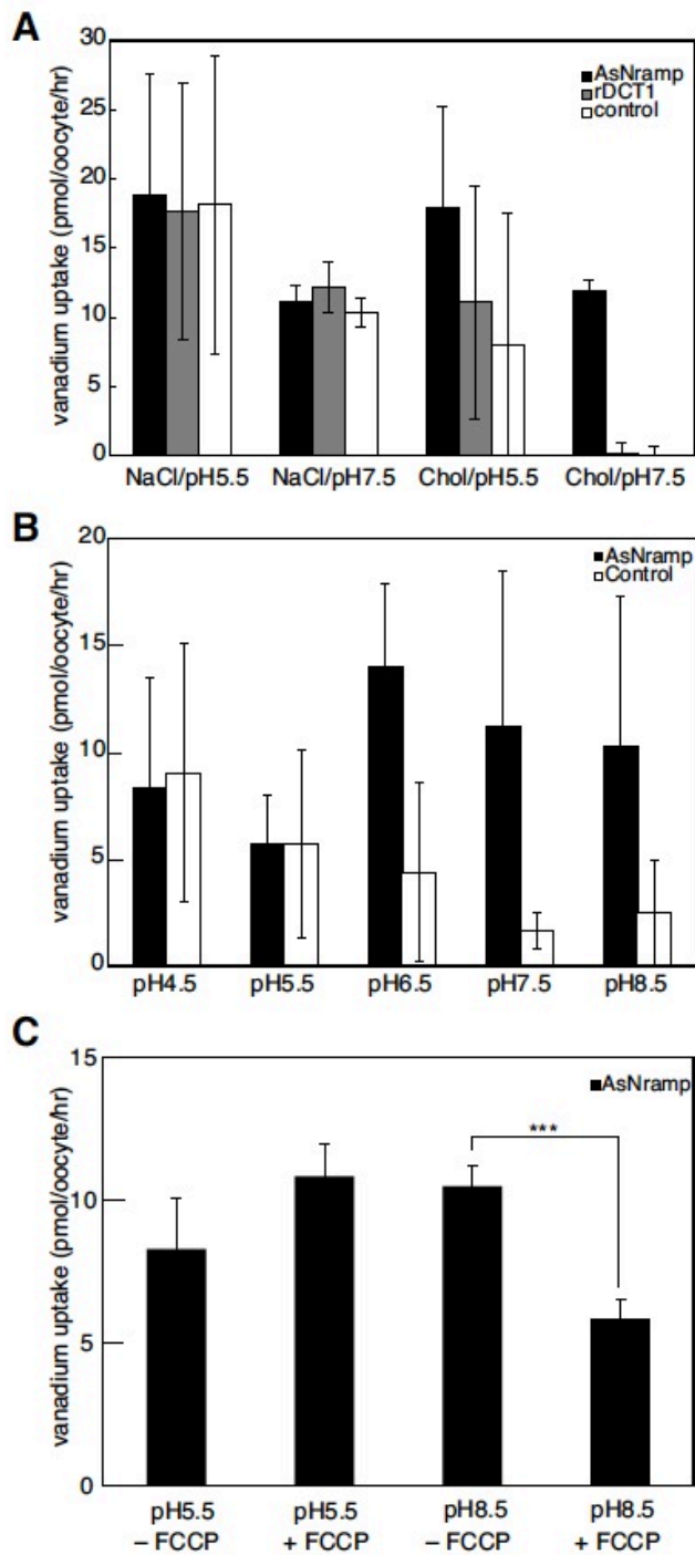
Fig. 5. Specificity of vanadium uptake by AsNramp and rat DCT1 in Xenopus oocytes. Oocytes were injected with 30–36 ng of AsNramp (solid bars) or rat DCT1 (gray bars) mRNA per oocyte and incubated for 4 days in MBS buffer before the uptake experiment. Control oocytes (open bars) were prepared at the same time and incubated in MBS buffer. A) VO^{2+} uptake was examined in a basal buffer
