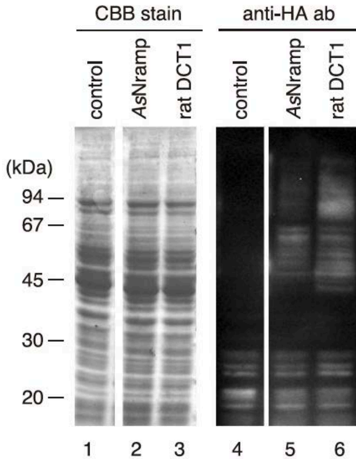
Fig. 4. Western blotting analysis of Xenopus oocytes injected with AsNramp or rat DCT1 mRNA. After SDS-PAGE, the gels were either stained with Coomassie Brilliant Blue (lanes 1–3), or the protein bands were transferred onto nitrocellulose membranes and probed with anti-HA antibody (lanes 4–6). Lanes 1 and 4, extract from control Xenopus oocytes; lanes 2 and 5, extract from oocytes injected with AsNramp mRNA; lanes 3 and 6, extract from oocytes injected with rat DCT1 mRNA. Note the broad signal from 45 kDa to more than 100 kDa detected only in oocytes injected with AsNramp or rat DCT1 mRNA (lanes 5 and 6).
