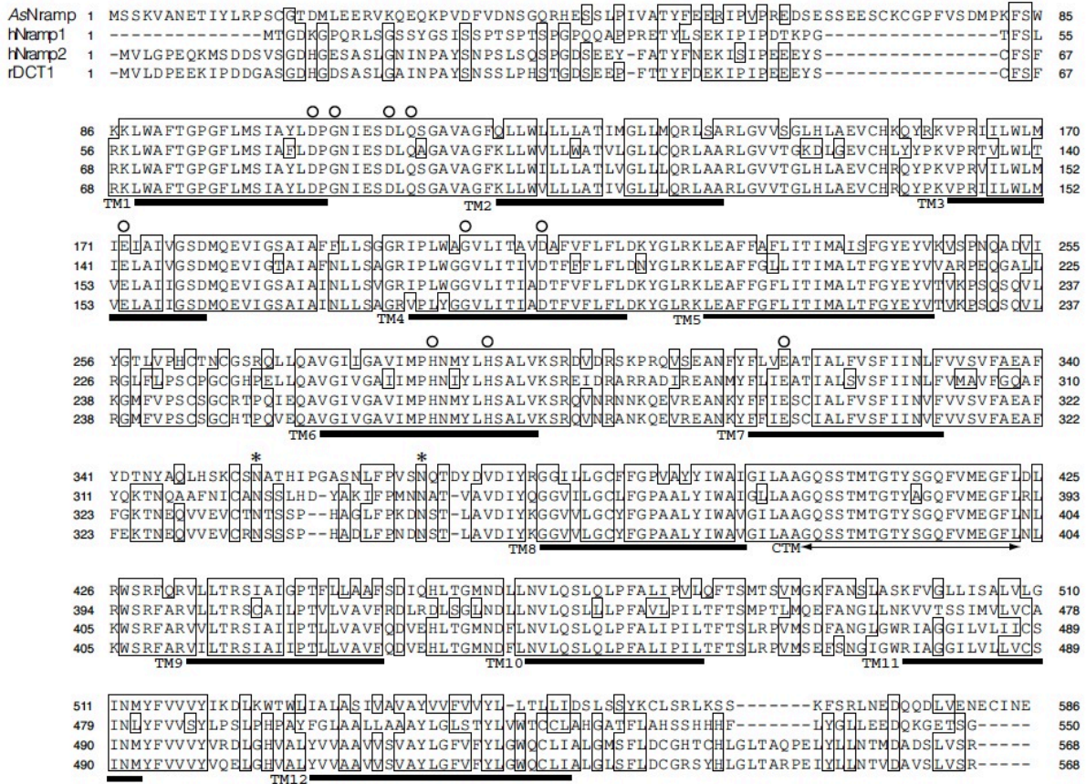
Fig. 1. Amino acid sequence alignment of an Nramp homolog of Ascidia sydneiensis samea (AsNramp), human Nramp1 (hNramp1), Nramp2 (hNramp2) and rat DCT1 (rDCT1). Identical amino acid residues are boxed. Twelve putative transmembrane domains are shaded (TM1 to TM12). Numbers indicate amino acid residues for each sequence. Open circles over each amino acid residue indicate identical ones that have been reported to be functionally essential or important. Asterisks indicate the position of possible N-glycosilation sites. Conserved transport motif is indicated by a double-headed arrow (CTM).
