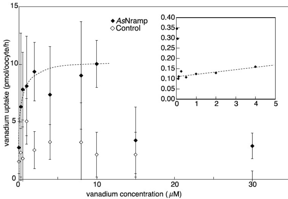
Fig. 7. Kinetic properties of vanadium uptake by AsNramp. Vanadium uptake was measured with increasing concentrations of \text{VO}^{2+} in uptake buffer (10 mM HEPES, 2 mM MES, 2 mM KCl, 1 mM \text{CaCl}_2 , 1 mM \text{MgCl}_2 , pH 8.5) containing 100 mM choline chloride. Each data point represents the mean value \pm SD ( n = 5 ). Calculated from the data between 0 and 10 \mu\text{M} , the K_m and V_{\max} of AsNramp were 90 nM and 9.1 pmol/oocyte/h, respectively, under these conditions (dotted lines).
