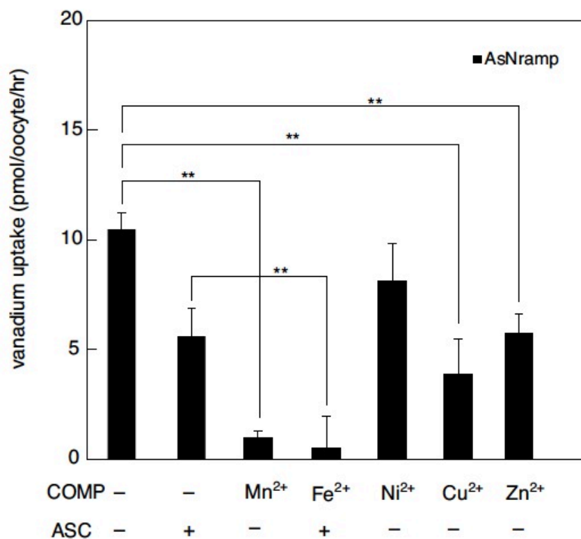
Fig. 6. The inhibition of \text{VO}^{2+} -uptake by AsNramp by excess divalent cations. Oocytes were injected with 32 ng of AsNramp mRNA per oocyte and incubated for 4 days before the uptake experiment. \text{VO}^{2+} uptake was examined in basal buffer (10 mM HEPES, 2 mM MES, 2 mM KCl, 1 mM \text{CaCl}_2 , 1 mM \text{MgCl}_2 , pH 8.5) supplemented with 100 mM choline chloride at 20°C. The initial \text{VO}^{2+} concentration was 10.5 \mu\text{M} , and the concentration of competitive divalent cations (COMP) were 525 \mu\text{M} (50 molar excess). Ascorbic acid (ASC) was added at 2.1 mM (4 molar excess) for control and \text{Fe}^{2+} . Bars indicate means \pm SE ( n = 10\text{--}12 ). *, P < 0.05 ; **, P < 0.01 .
