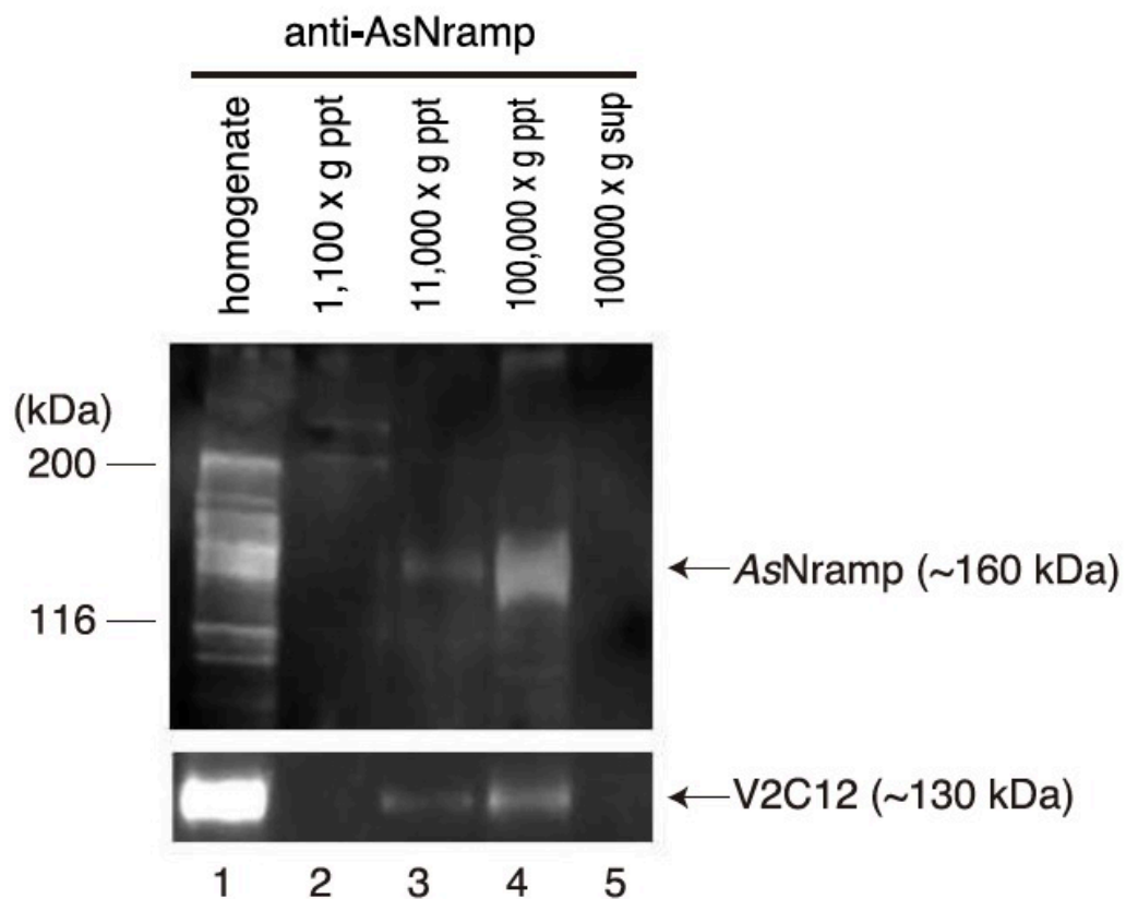
Fig. 3. Expression of AsNramp protein identified by anti- AsNramp antiserum on a Western blot after fractionation. Samples were separated by 8% SDS-PAGE. After electrophoresis, the gels were transferred onto nitrocellulose membranes and reacted with 1:4000 dilution of anti- AsNramp antiserum. Lane 1, homogenate blood cells without giant cells; lane 2, pellet obtained by centrifugation at 1100 × g; lane 3, pellet obtained by centrifugation at 11,000 × g; lane 4, pellet obtained by centrifugation at 100,000 × g; lane 5, soluble protein. V2C12 recognizes a 130-kDa vacuolar membrane protein. Note that an AsNramp signal (~160 kDa) was detected in the vacuolar membrane fraction (lane 4).
