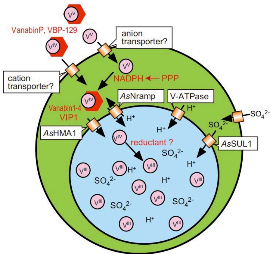
Fig. 8. A model for vanadium transport in vanadocytes of the vanadium-rich ascidian Ascidia sydneiensis samea . Vanadium ions are transported by an anion transporter (for V^V ) or cation transporter (for V^{IV} ) into the cytoplasm of vanadocytes. V^V is reduced to V^{IV} through an electron transfer cascade from the electron donor, NADPH, via glutathione reductase, glutathione, and Vanabin2 [19]. The vacuole content is acidified by V-ATPase, and AsSUL1 accumulates sulfate ions. P_{1B} -type ATPase, AsHMA1, and/or a proton/ V^{IV} antiporter, AsNramp, transports V^{IV} into the vacuole. V^{IV} is reduced to V^{III} by an as yet unknown reductant and stabilized in acidic solution, in which sulfate ions exist as counterions for V^{III} . Reproduced from [45] with permission from the copyright holders.
