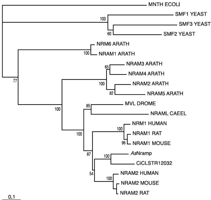
Fig. 2. Phylogenetic tree using the neighbor-joining method based on amino acid sequences of Nramp family proteins. Two ascidian species ( AsNrap and CiCLSTR12032 , from Ascidia sydneiensis samea and Ciona intestinalis , respectively) were compared with homologs from representative organisms. Labels are taken from SwissProt database IDs (ECOLI, Escherichia coli ; YEAST, Saccharomyces cerevisiae ; ARATH, Arabidopsis thaliana ; DROME, Drosophila melanogaster ; CAEEL, Caenorhabditis elegans ; HUMAN, Homo sapiens ; RAT, Rattus norvegicus ; MOUSE, Mus musculus ). The scale bar indicates 0.1 amino acid substitutions per site. Numbers at each branch indicate the percentage of times that a node was supported in 1000 bootstrap pseudoreplicates. Note that two ascidian species were clearly clustered, but they were not significantly clustered to either Nramp1 or Nramp2.
