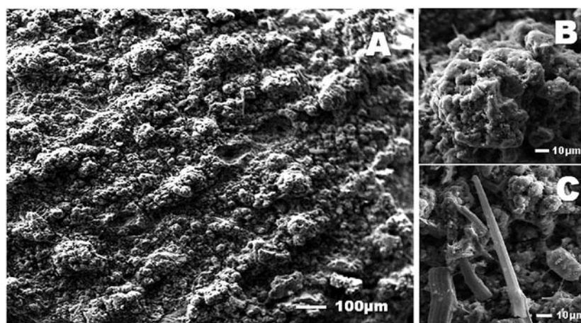
Fig.3. Scanning electron micrographs of deposited material on the shell surface of Phenacolepas pulchella . A, Cauliflower-like, 60- \mu\text{m} -wide deposits are precipitated along apical radial ridges of the shell. B, magnified view of a deposit, which appears as an amorphous porous aggregate. C, dead diatom frustules in the aggregate.
