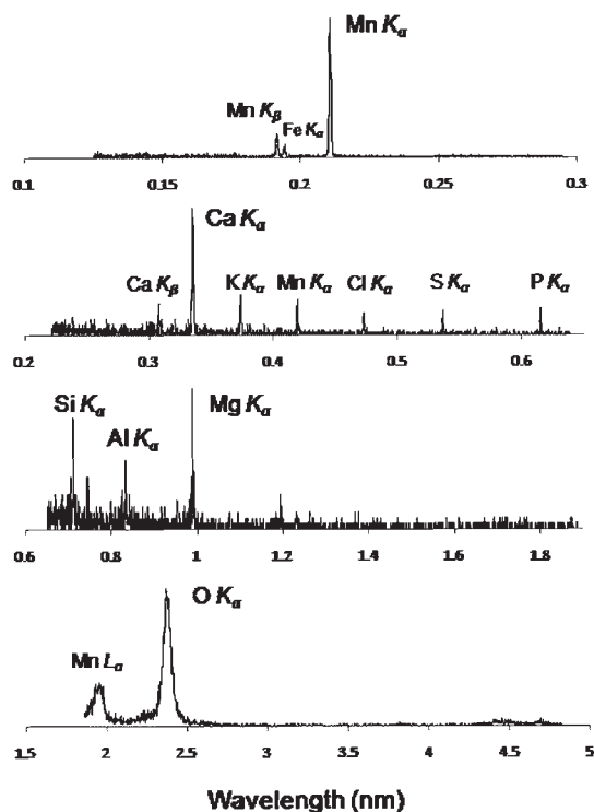
Fig.5. Fluorescence X-ray spectra of the deposits on the shell surface of Phenacolepas pulchella . X-axis shows wavelengths in nanometers (nm), while intensities are exhibited in arbitrary units. Peaks corresponding to specific elements were detected. The X-ray spectroscopy was done using different analyzing crystals.
