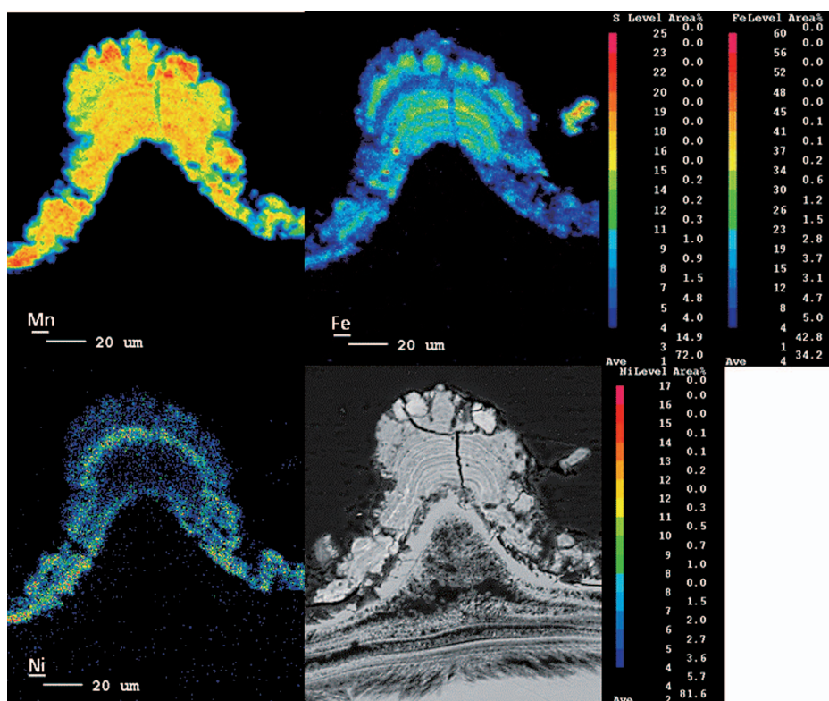
Fig.6. Mapping of Mn (upper left), Fe (upper right), and Ni (lower left), and back-scattered electron image (lower right) of a deposit on the shell surface of Phenacolepas pulchella . Warmer and cooler colors indicate relatively higher and lower abundances, respectively.
