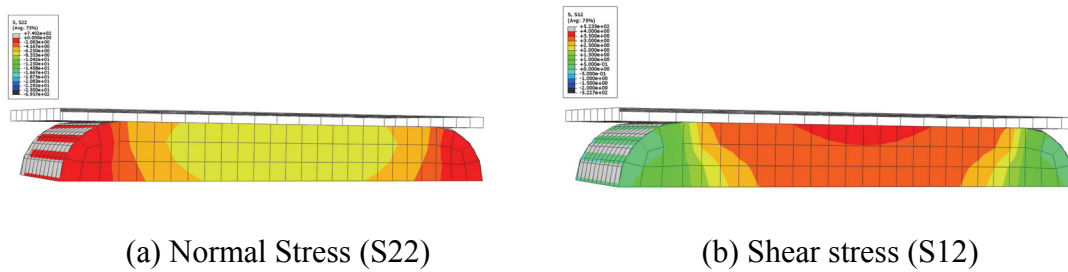
Fig 14. Filled contours of measured stress components within the granular material (unit: kPa)
