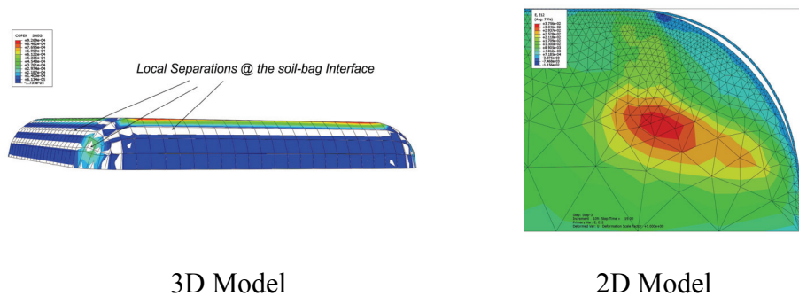
Fig 12. Local separation-reclosure at the soil-bag interface during the cyclic shear test.
