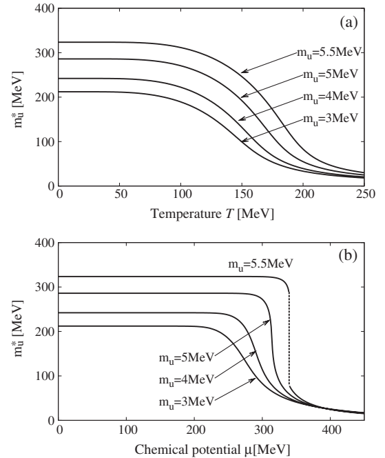
FIG. 5. m_u^* in the case of cutoff. (a) finite T and \mu = 0 ; (b) finite \mu and T = 10 MeV.
