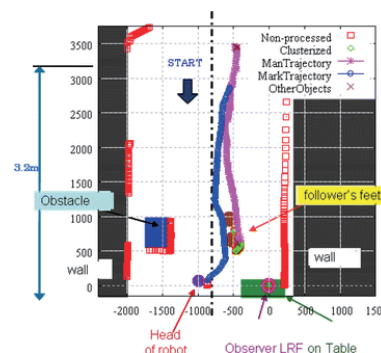
Fig. 2 Trace of the robot and follower
