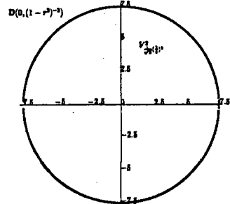
Figure 3.4: r = 0.8
