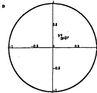
Figure 3.2: r = 0.06
