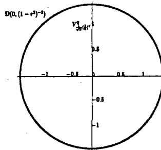
Figure 3.3: r = 0.4
