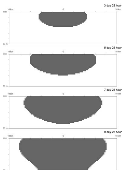
Figure 5. Calculated distributions of the influence area of high turbidity waters (Case 2). The shadow area denotes that the concentration of suspended sediment is higher than 5.0 \text{ mg L}^{-1} .
