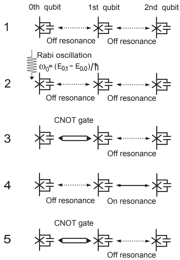
Fig. 6. Procedure for generating the GHZ state by using CNOT gate operations. The Rabi oscillation step depicted above corresponds to a \pi/2 rotation.
