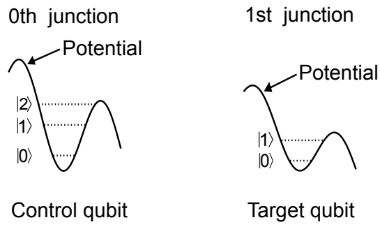
Fig. 4. Schematic diagram of the effective potential for the control and target qubits for the CNOT gate.
