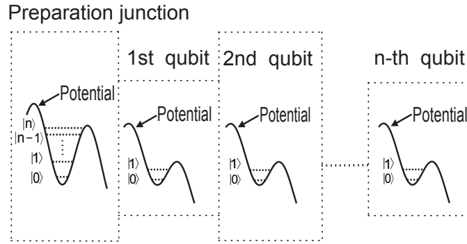
Fig. 2. Schematic diagram of the (tilted-washboard) effective potential for the phase variable of the preparation junction and the n qubits. The dotted lines represent the quantum states that will be used below.
