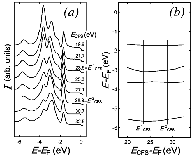
FIG. 10. A constant- \mathbf{K}_{\parallel} series of CFS spectra (a) and the dispersion of the main peaks (b) on varying the final-state energy E_{\text{CFS}} through a E^1_{\text{CFS}} -to- E^2_{\text{CFS}} discontinuity of its dispersion determined by VLEED (Fig. 4) for K_{\parallel} = 1.5 \text{ \AA}^{-1} in the \Gamma \bar{X} azimuth. The peak energies are almost constant through the discontinuity.
