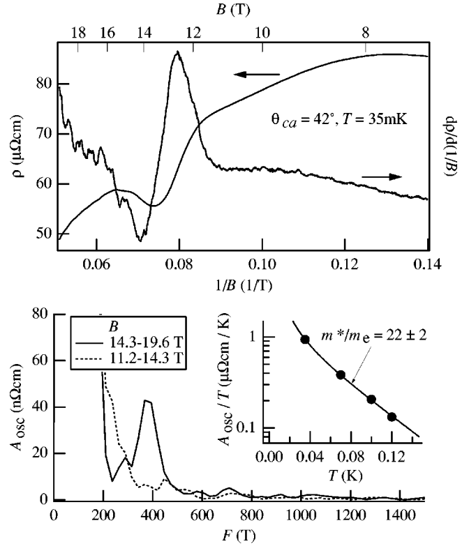
FIG. 5. (a) Resistivity \rho in CeNiSn for the field angle \theta_{ca} = 42^\circ and its derivative with respect to the inverse field 1/B as functions of 1/B . The magnetoresistance decreases fairly sharply from 12 T and exhibits a dip at 13.5 T. The derivative curve indicates the existence of SdH oscillations above this dip. (b) The Fourier spectra for field ranges above (solid curve) and below (dashed curve) the magnetoresistance dip. The inset shows the temperature dependence of the amplitude A_{\text{osc}} of SdH oscillations observed above the dip.
