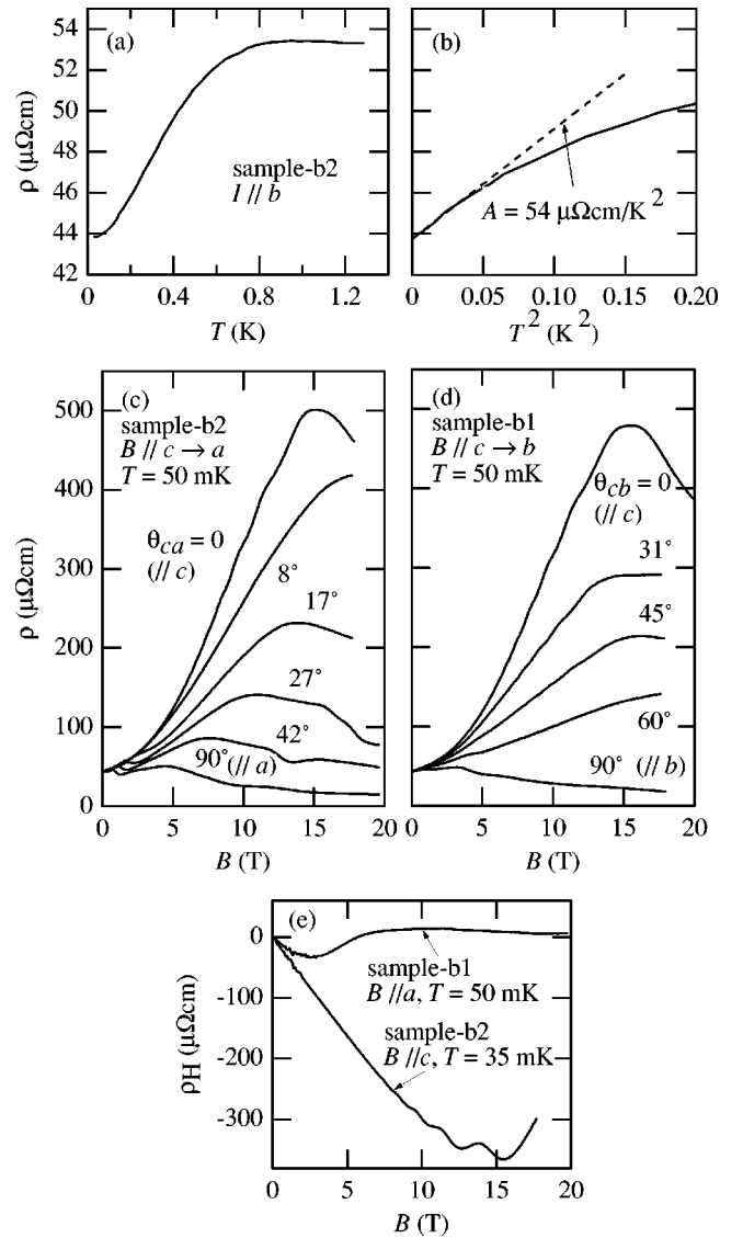
FIG. 1. (a) Resistivity \rho in \text{CeNiSn} measured along the b axis as a function of temperature T . (b) Low-temperature part of the same data as a function of T^2 . The dashed line shows a fit to \rho = \rho_0 + AT^2 below 0.16 K. (c) and (d) \rho vs field B for selected field directions in the ac and bc planes, respectively. The field angles \theta_{ca} and \theta_{cb} are measured from the c axis. Note that the field geometry is always transverse in (c), while it changes from transverse at \theta_{cb} = 0 to longitudinal at \theta_{cb} = 90^\circ in (d). (e) Hall resistivity \rho_H vs B for B \parallel a and B \parallel c .
