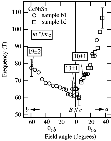
FIG. 4. The field-direction dependence of the SdH frequency in CeNiSn. The frequencies were determined from Fourier transforms of oscillations in the following field intervals: B = 5.56\text{--}14.3 T for all \theta_{cb} 's and for \theta_{ca} < 26^\circ and B = 5.56\text{--}10.9 T for \theta_{ca} \geq 26^\circ . For the ac plane, the measurements on the two samples yielded identical results within experimental error (compare the circles and squares). The effective mass is also shown for selected field directions.
