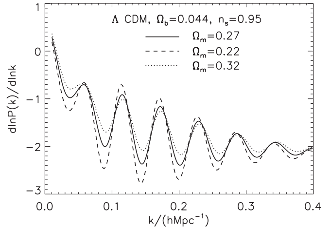
FIG. 4. Theoretical curves of d \ln P / d \ln k in the \Lambda CDM model showing the effect of changing \Omega_m : the solid curve has \Omega_m = 0.27 , the dashed curve has \Omega_m = 0.22 , the dotted curve has \Omega_m = 0.32 . The other parameters are the same as those of Fig. 3, n_s = 0.95 and \Omega_b = 0.044 .
