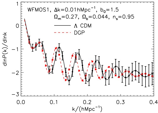
FIG. 9 (color online). Theoretical predictions for d \ln P / d \ln k assuming the sample WFMO S1 (corresponding to z < 1.3 ). The squares with error bar are evaluated with the simple simulation of the power spectrum for the \Lambda CDM model. The asterisks are the DGP model, but the error bar, which is almost the same as that of the \Lambda CDM model, is omitted for simplicity. Theoretical curves are the DGP model (dashed curve) and the \Lambda CDM model (solid curve). The parameters are the same as those in Fig. 3, i.e., n_s = 0.95 , \Omega_b = 0.044 , \Omega_m = 0.27 , and b_0 = 1.5 . Here we used the nearest two points in the differentiation and \Delta k = 0.01 h \text{ Mpc}^{-1} .
