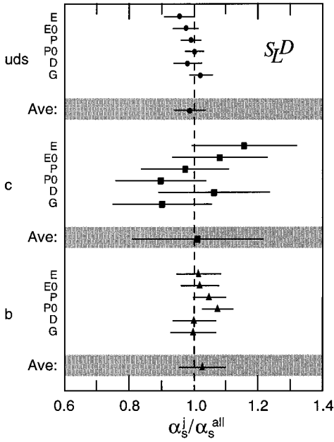
FIG. 2. Values of \alpha_s^j/\alpha_s^{\text{all}} derived for each of the six jet algorithms for each of the quark flavors j (see text). The error bars on the averages include the statistical and systematic errors and the total theoretical uncertainty.
