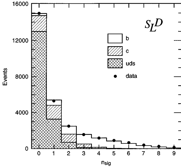
FIG. 1. The measured distribution of the number of tracks per event with d/\sigma_d \geq 3.0 (points). The histograms show the flavor composition estimated from a Monte Carlo simulation (see text).
