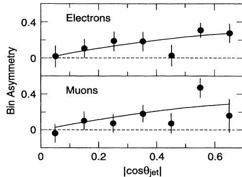
FIG. 2. Experimentally observed left-right forward-backward asymmetry \hat{A}_{FB}^b (data points with statistical errors); theoretical asymmetry function |P_e|A_b 2z/(1+z^2) fit to data (solid curve).
