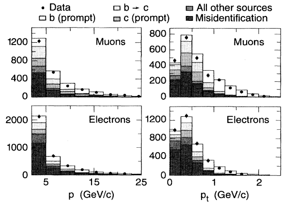
FIG. 1. Distributions of momentum and transverse momentum with respect to the nearest jet axis for identified electrons and muons in the data (points), compared to the MC prediction (histograms) for various sources.
