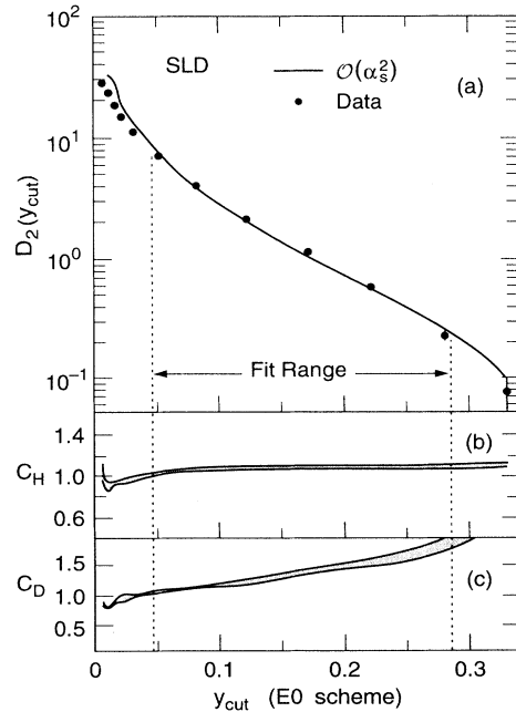
FIG. 23. The same as Fig. 16 but for the differential two-jet rate with the E0 scheme.
