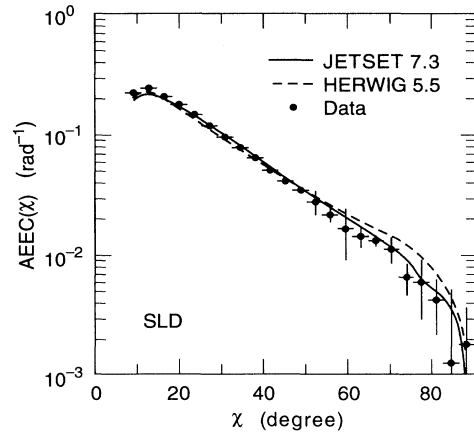
FIG. 14. The same as Fig. 1 but for the asymmetry of the energy-energy correlation (AEEC).
