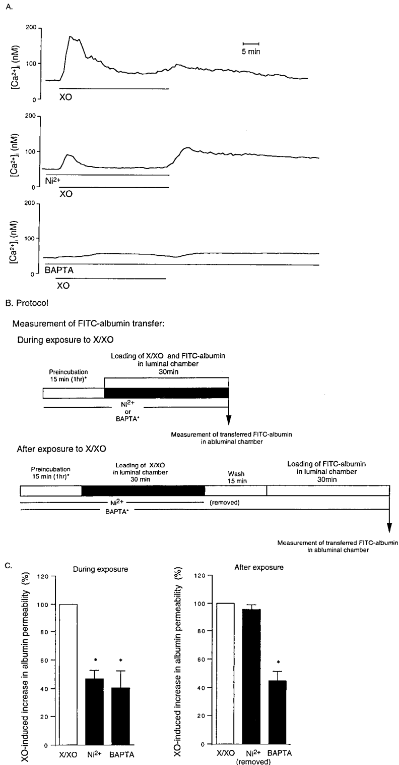
Fig. 3. (A) Representative recordings of cytosolic \text{Ca}^{2+} movement of porcine pulmonary artery endothelial (PPAE) cells during and after the exposure to 200 \mu\text{M} xanthine and 0.04 U/ml xanthine oxidase (X/O). Intracellular concentration of \text{Ca}^{2+} ( [\text{Ca}^{2+}]_i ) was measured at 37°C by using Fura-2 fluoremetry. Upper trace: X/O was removed after a 30-min exposure. Middle trace: same condition as in the upper trace except that PPAE cells were exposed to X/O in the presence of 1.5 mM \text{Ni}^{2+} . \text{Ni}^{2+} was removed together with X/O. Lower trace: same condition as in the upper trace except that PPAE cells were pre-loaded with 5 \mu\text{M} BAPTA/AM. (B) Experimental protocol to examine the albumin permeability, examined as the concentration of 5 mg/ml (FITC)-albumin transferred: (1) during exposure of PPAE cells to X/O for 30 min at 37°C; and (2) during the 30-min incubation period following the 30-min X/O exposure. *Preincubation time for BAPTA/AM was 1 hour. (C) Percent change, assuming albumin permeability in the absence or presence of X/O exposure to be 0% and 100%, respectively. Data are expressed as mean \pm SE of 4–6 separate experiments. PPAE cells used were obtained from at least three separate cell lines. *Significant difference from X/O ( p < 0.05 ).
