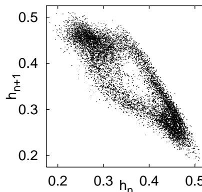
FIG. 1. A return map of the collective motion in GCM (1) without noise. a = 1.86 , \epsilon = 0.1 , \sigma = 0.0 , N = 10^7 .
