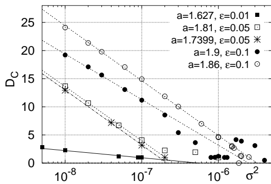
FIG. 3. The dimension of the collective motion is plotted as a function of noise intensity, obtained by the Lyapunov dimension. The Lyapunov exponents are calculated as growth rates of the tangent vector around the orbit, obtained by Eq. (4). For numerical calculation, \rho_n(x) is approximated by a sufficiently large dimensional vector, and the tangent vectors are orthonormalized at each time step.
