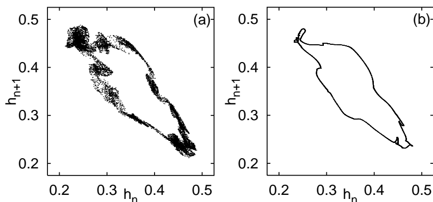
FIG. 2. Return maps of the collective motion in GCM (1) with noise. a = 1.86 and \epsilon = 0.1 . The noise variances are (a) \sigma^2 = 1.5 \times 10^{-6} and (b) \sigma^2 = 2.7 \times 10^{-6} . The Lyapunov dimension for (a) is estimated at 3.08. Numerical calculation was carried out with integration of Eq. (4) using a sufficiently large dimensional vector to approximate the distribution function. When the system size in Fig. 1 is sufficiently large and the noise in this figure is small enough, the difference between these are expected not to be significant.
