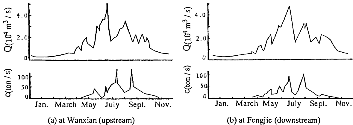
Fig.1 Hydrograph and Suspended-load Curves from the Yangtze River (Ning Chien et al.1987, p.75)
