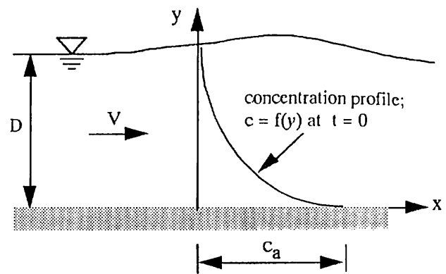
Fig.2 Definition Sketch
