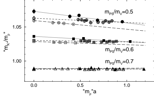
Figure 2. Fictitious mass ratio “ m_{K^*}/m_{\rho} ” defined in the text at different sea quark masses. Filled, thick open and thin open symbols are the results from RC , qRC and qPW simulations, respectively.
