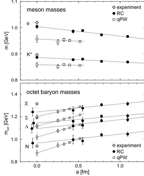
Figure 1. Typical hadron masses with m_K -input.
