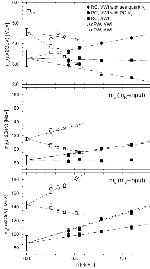
Figure 3. Continuum extrapolation of m_{ud} (top) and m_s with m_K -input(middle) and m_{\phi} -input(bottom).
