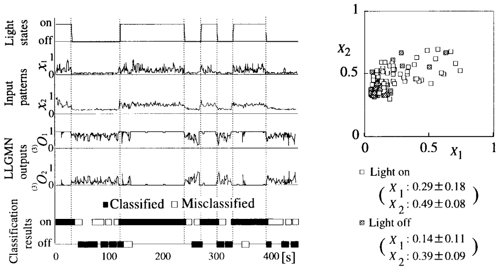
Fig. 11. Classification results under the artificial photic stimulation by LLGMN.
